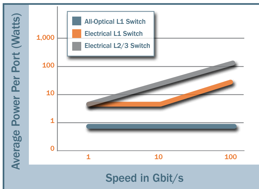
FIGURE 4. Average power based on increase in speed
