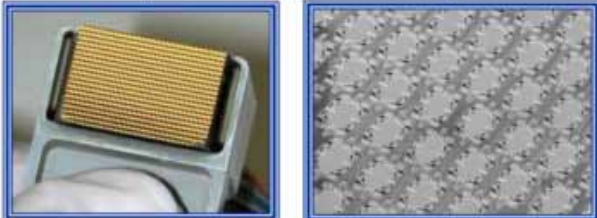
Collimator Lens Array and MEMS Element.
